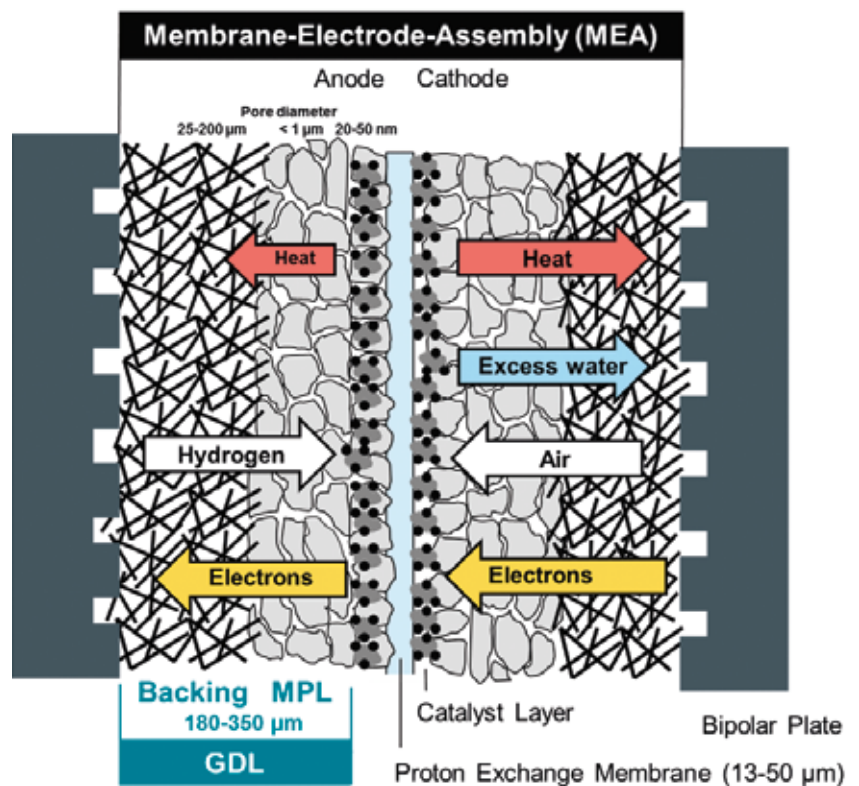
↑ Sketch of a single cell fuel cell with gas diffusion layers (GDL)
